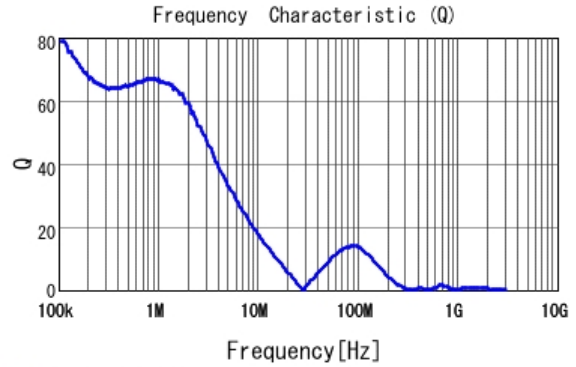
■ FDSD0630-H-3R3M Q
