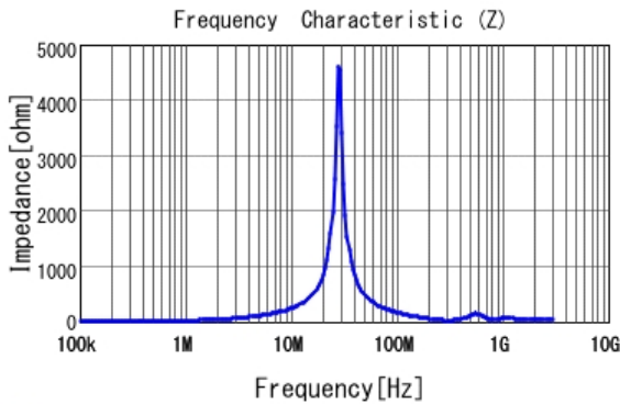
■ FDSD0630-H-3R3M |Z|
