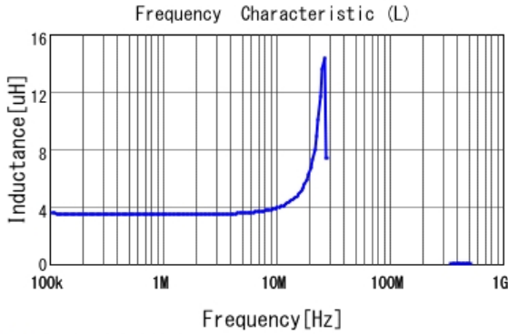
■ FDSD0630-H-3R3M L
