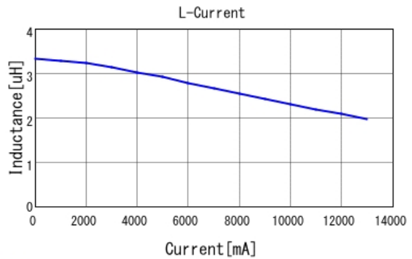
■ FDSD0630-H-3R3M L-Current 20degC
